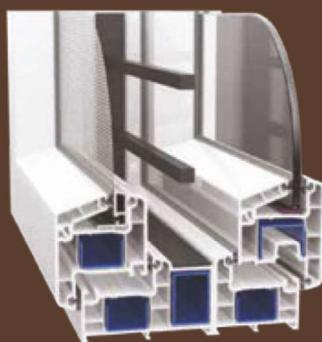
Casement Window with Grill and Mesh
